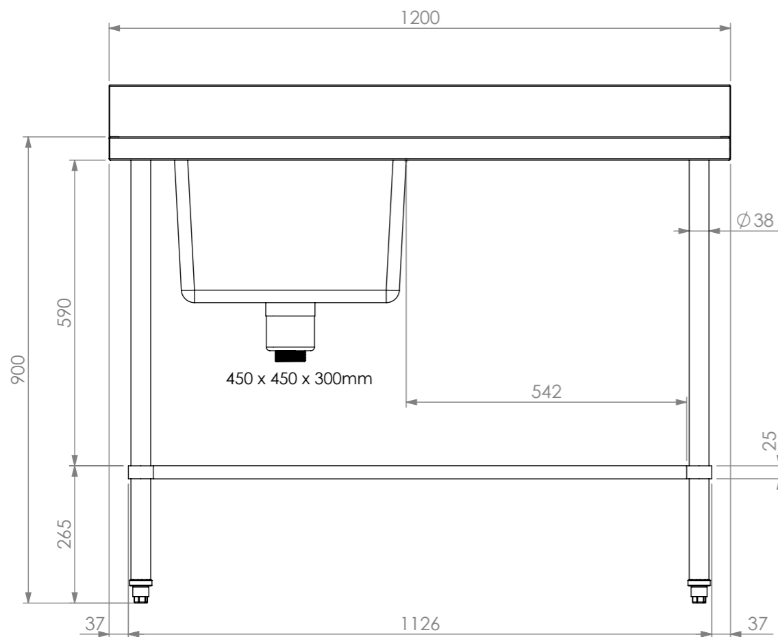
FRONT ELEVATION
